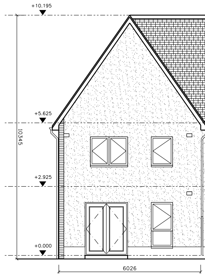
REAR ELEVATION
