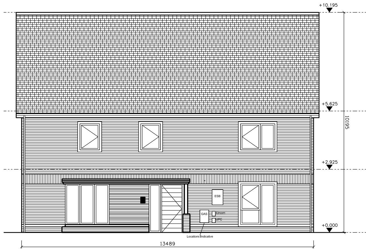
SIDE ELEVATION
